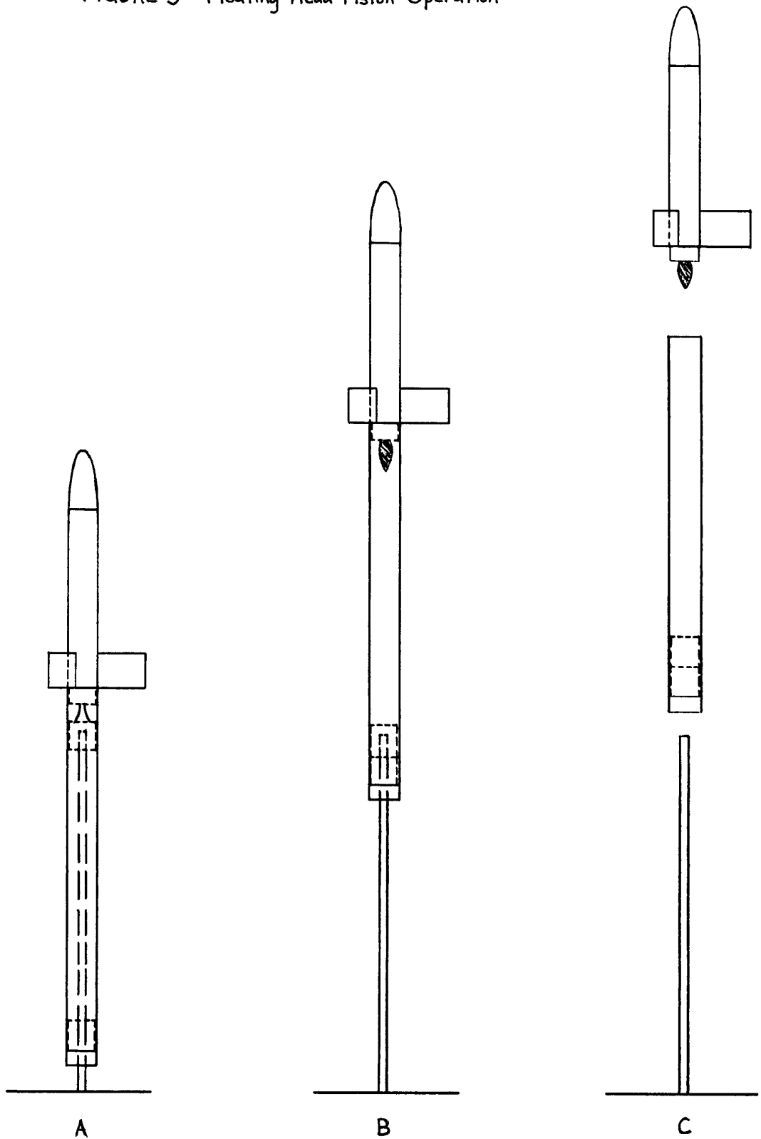
FIGURE 3 - Floating Head Piston Operation
