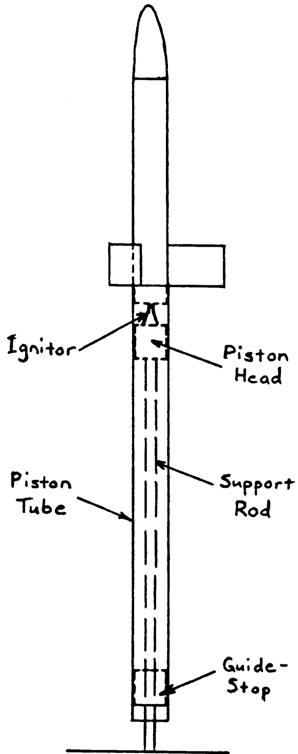
FIGURE 1 - Piston Nomenclature
